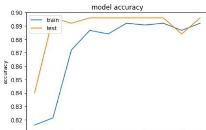
Fig. 3. Graph of model accuracy
