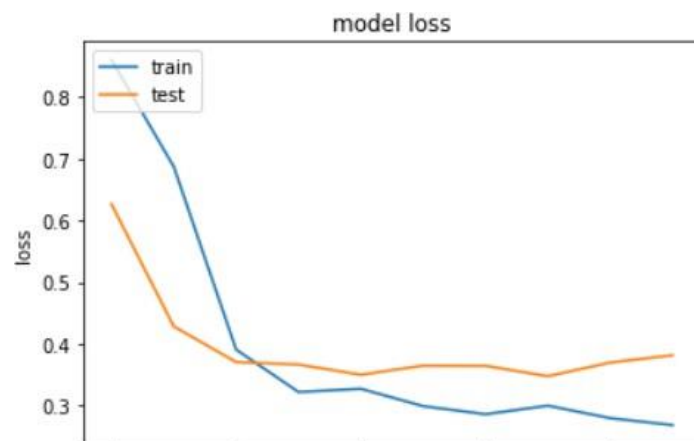
Fig. 4. Graph of the loss function
